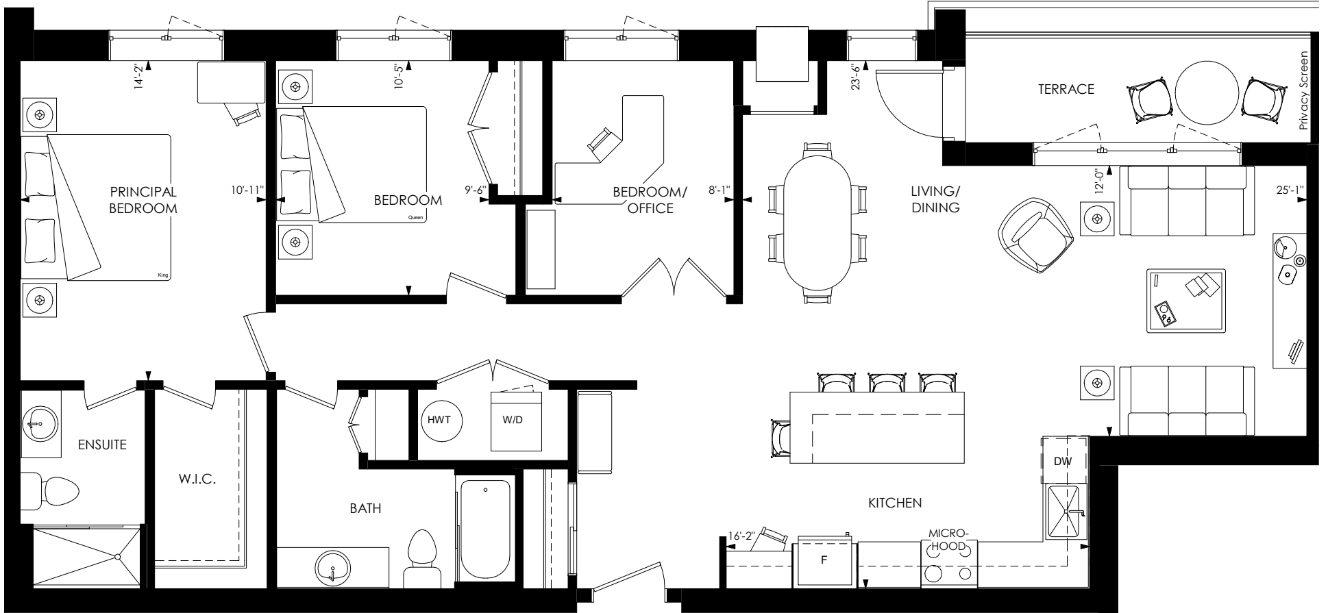
Unit Type J - 2 Bedroom + Bedroom/Office - 1331 sq. ft.
