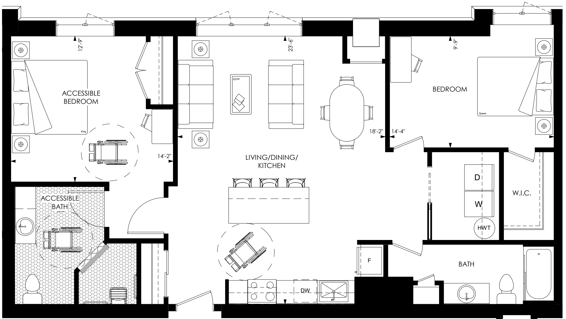
Unit Type K - 2 Bedroom Universal - 1233 sq. ft.
